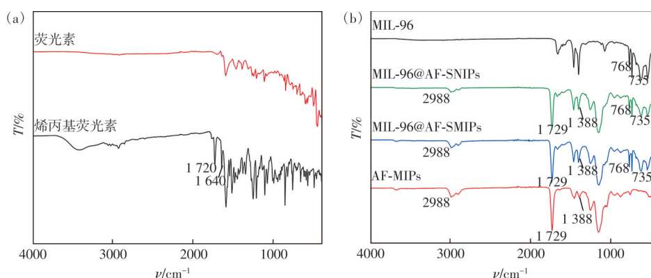
图1 (a)荧光素和烯丙基荧光素的红外光谱;(b)MIL-96、MIL-96@AF-SNIPs、MIL-96@AF-SMIPs和AF-MIPs的红外光谱 Fig.1 (a) FTIR images of fluorescein and allylfluorescein. (b) FTIR images of MIL-96, MIL-96@AF-SNIPs, MIL-96@AF-SMIPs and AF-MIPs
