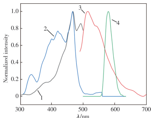
图6 归一化后MIL-96@AF-SMIPs的荧光激发(1)和发射(3)光谱与罗丹明B的荧光激发(2)和发射(4)光谱 Fig.6 Normalized fluorescence excitation (1) and emission (3) spectra of MIL-96@AF-SMIPs and fluorescence excitation (2) and emission (4) spectra of Rhodamine B
