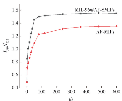
图7 MIL-96@AF-SMIPs与AF-MIPs的吸附速率对比 Fig.7 Comparison of adsorption rates between MIL-96@AF-SMIPs and AF-MIPs
